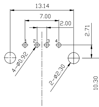
RECOMMENDED P.C.B. PATTERN LAYOUT
