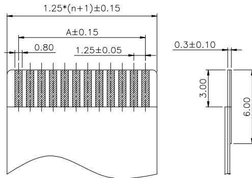
(Tolerance:0.05) FFC/FPC Dimension T=0.3mm
