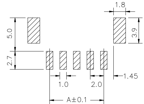
RECOMMENDED P.C. BOARD LAYOUT DIMM.
