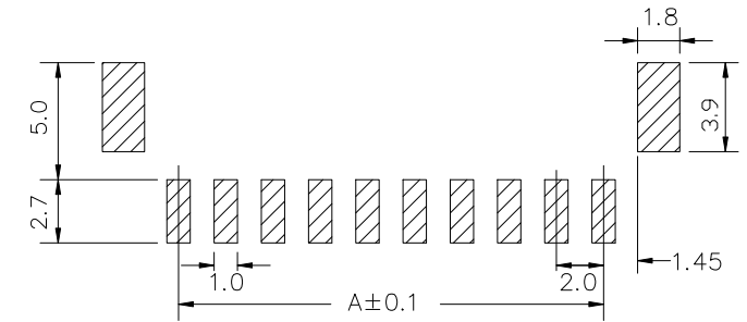
RECOMMENDED P.C. BOARD LAYOUT DIMM.
