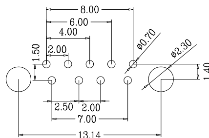
RECOMMENDED PCBA LAYOUT
