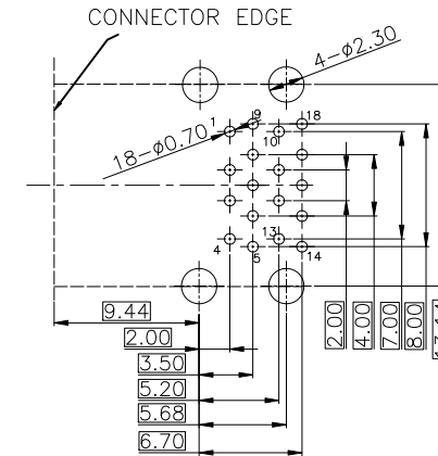
P.C.B. LAYOUT (COMPONENT SIDE) DEFAULT TOLERANCE: ±0.05
